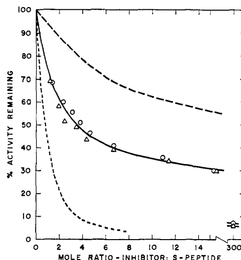
Figure 5. Inhibition of RNase S by FOrn 10 3-CMHis 12 S-peptide 1-14 (Δ) and Orn 10 3-CMHis 12 S-peptide 1-14 (○) with yeast RNA as substrate. Molar ratio of S-peptide to S-protein, 1:1. For comparison the inhibition curves for Orn 10 Pyr(3)ala 12 S-peptide 1-14 (— — —) and 3-CMHis 12 S-peptide 1-14 (---) are given.
