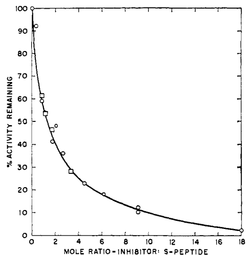
Figure 2. Competition of Pyr(3)ala 12 S-peptide 1-14 with natural S-peptide (O) and S-peptide 1-14 (o) for S-protein; substrate, yeast RNA. Molar ratio of either natural S-peptide or S-peptide 1-14 to S-protein, 1:1. Abscissa: molar ratio of inhibitor to S-peptide. Ordinate: per cent activity remaining. Reversal of inhibition by addition of increasing amounts of natural S-peptide to inhibited enzyme (□).
