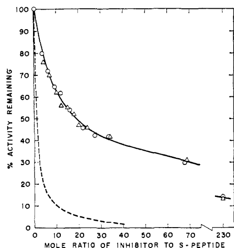
Figure 4. Inhibition of RNase S by FOrn 10 Pyr(3)ala 12 S-peptide 1-14 (Δ) and Orn 10 Pyr(3)ala 12 S-peptide 1-14 (○) with yeast RNA as substrate. Molar ratio of S-peptide to S-protein, 1:1. For comparison inhibition by Pyr(3)ala 12 S-peptide 1-14 (---) is given.
