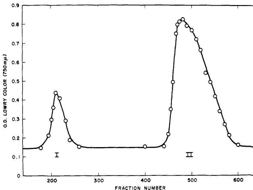
Figure 1. Separation of 1-CMHIS- (peak I) and 3-CM-histidylmethionylaspartic acid d -sulfoxide (peak II) on an AG 1-X2 column (1.9 × 60 cm); fraction size 2 ml.
